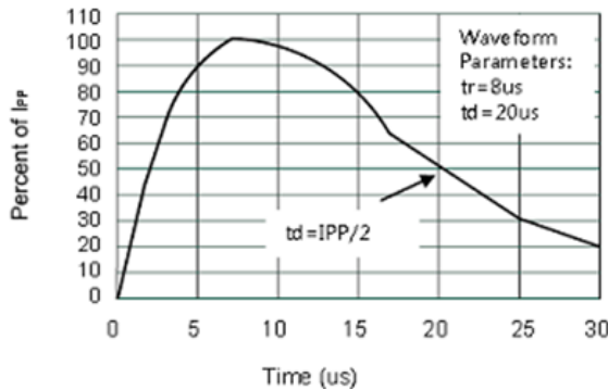
FIGURE 1 Pulse Waveform
